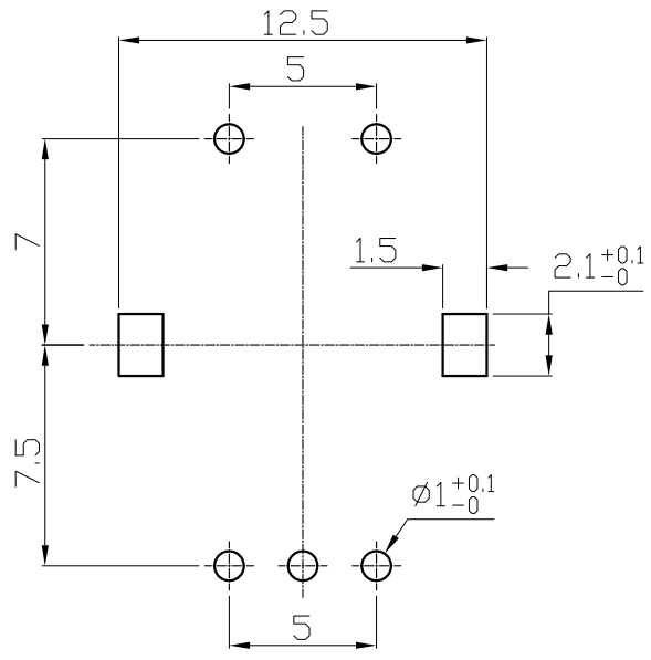
P.C.B.MOUNTING DETAIL
