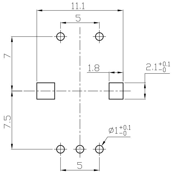
P.C.B.MOUNTING DETAIL
