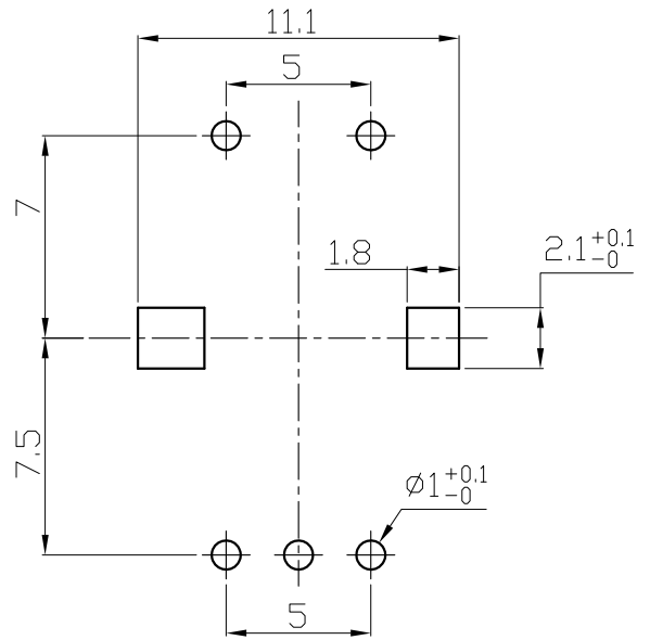
P.C.B.MOUNTING DETAIL
